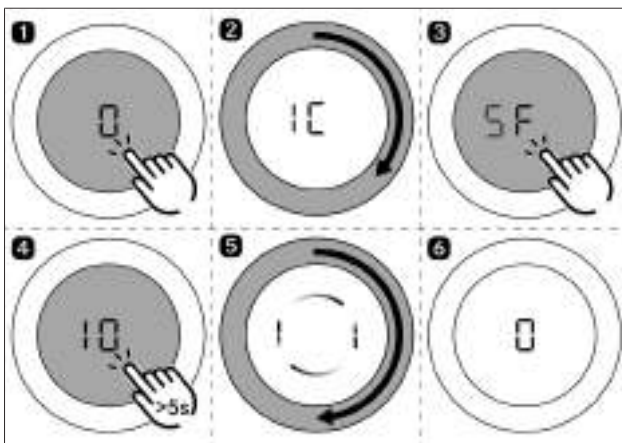
Fig. 5.21 Resetting the filter service life early
